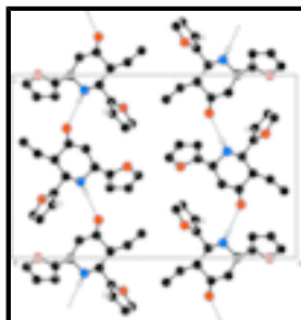
Fig. 2. The molecular packing of the title compound, viewed down the a axis showing the N—H···O (dashed lines) hydrogen bonds.
